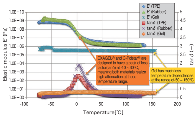
Dynamic Viscoelasticity Measurement (DMA, 30Hz)
